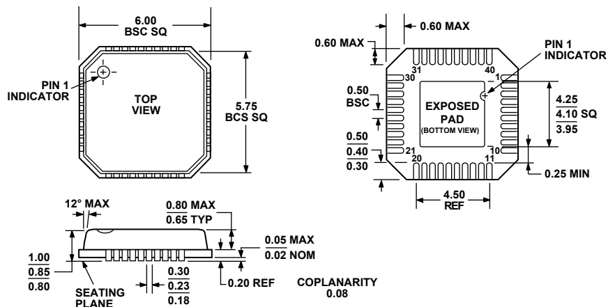
Figure 48. 40-Lead Lead Frame Chip Scale Package [LFCSP_VQ] 6 mm × 6 mm Body, Very Thin Quad (CP-40)
